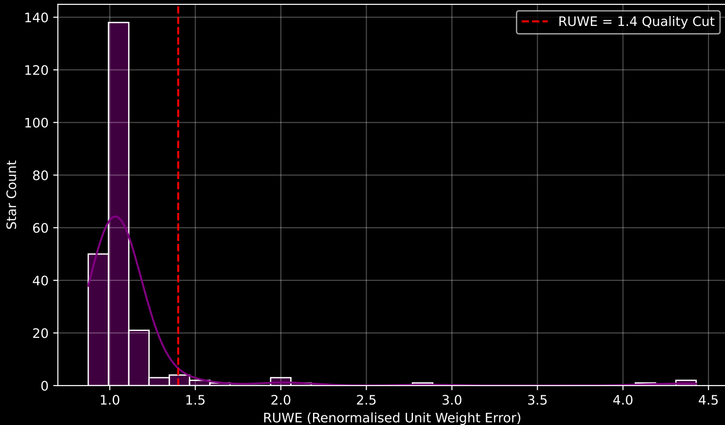
GAPOGEE DR17 Field [NGC7789_btx] RUWE Distribution (n= 227)
