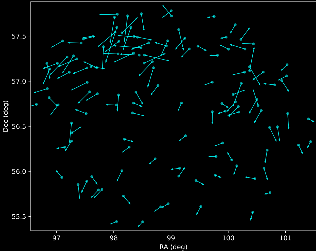
APOGEE DR17 Noise Stream Proper Motion Vectors (n=126)
