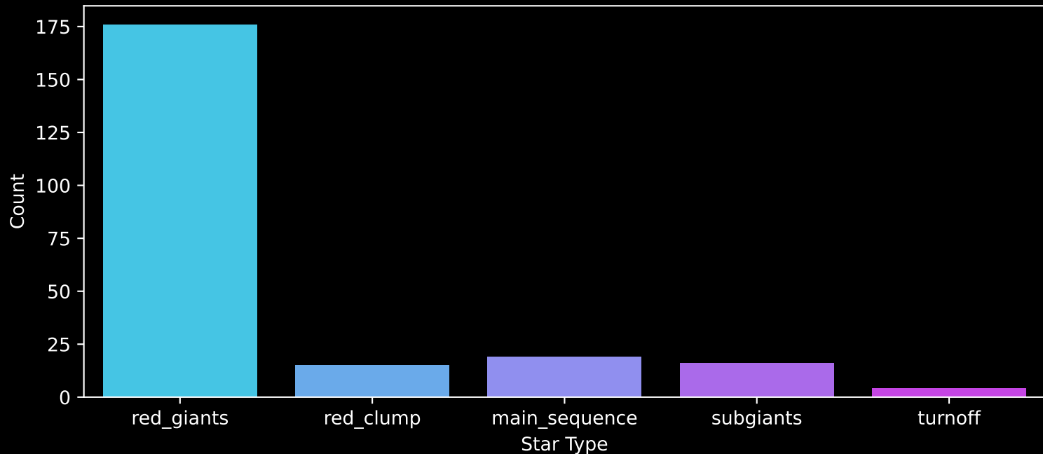
APOGEE DR17 Field: [NGC7789_btx] Count plot of Star Type
