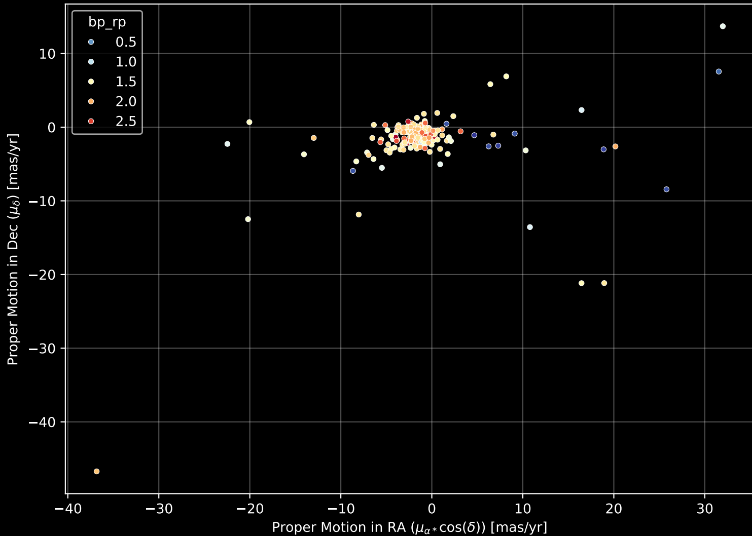
APOGEE DR17 Field: [NGC7789_btx] Proper Motion Diagram (n= 230)
