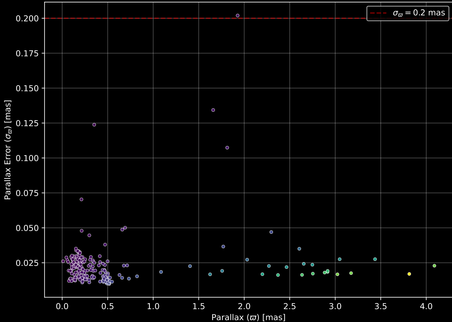
APOGEE DR17 Field: [NGC7789_btx] Parallax Quality (n= 230)
