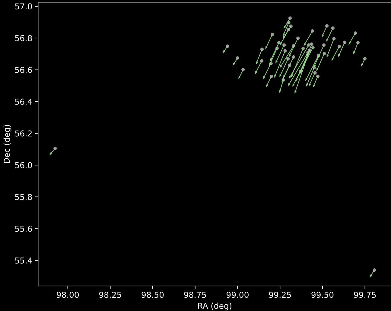
APOGEE DR17 Cluster 5 Proper Motion Vectors (n=47)
