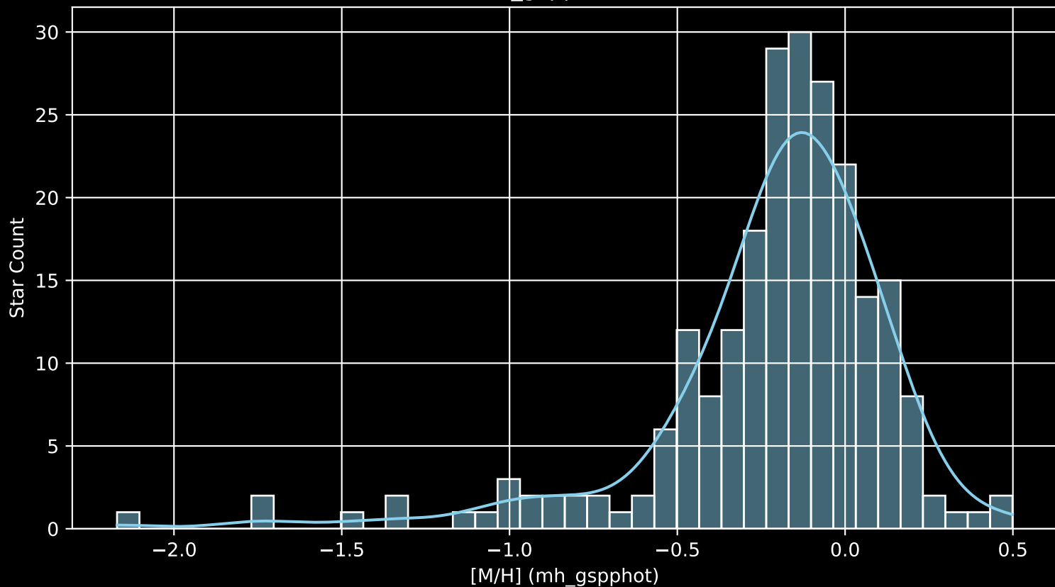
APOGEE DR17 Field: [NGC7789_btx [M/H] (mh_gspphot) (n= 229)
